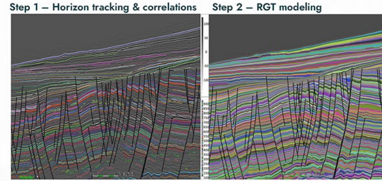
Phase 2 - RGT modeling framework from seismic reflections
