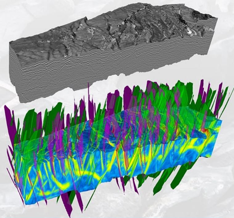
Phase 1 - Fault extraction from seismic amplitudes
